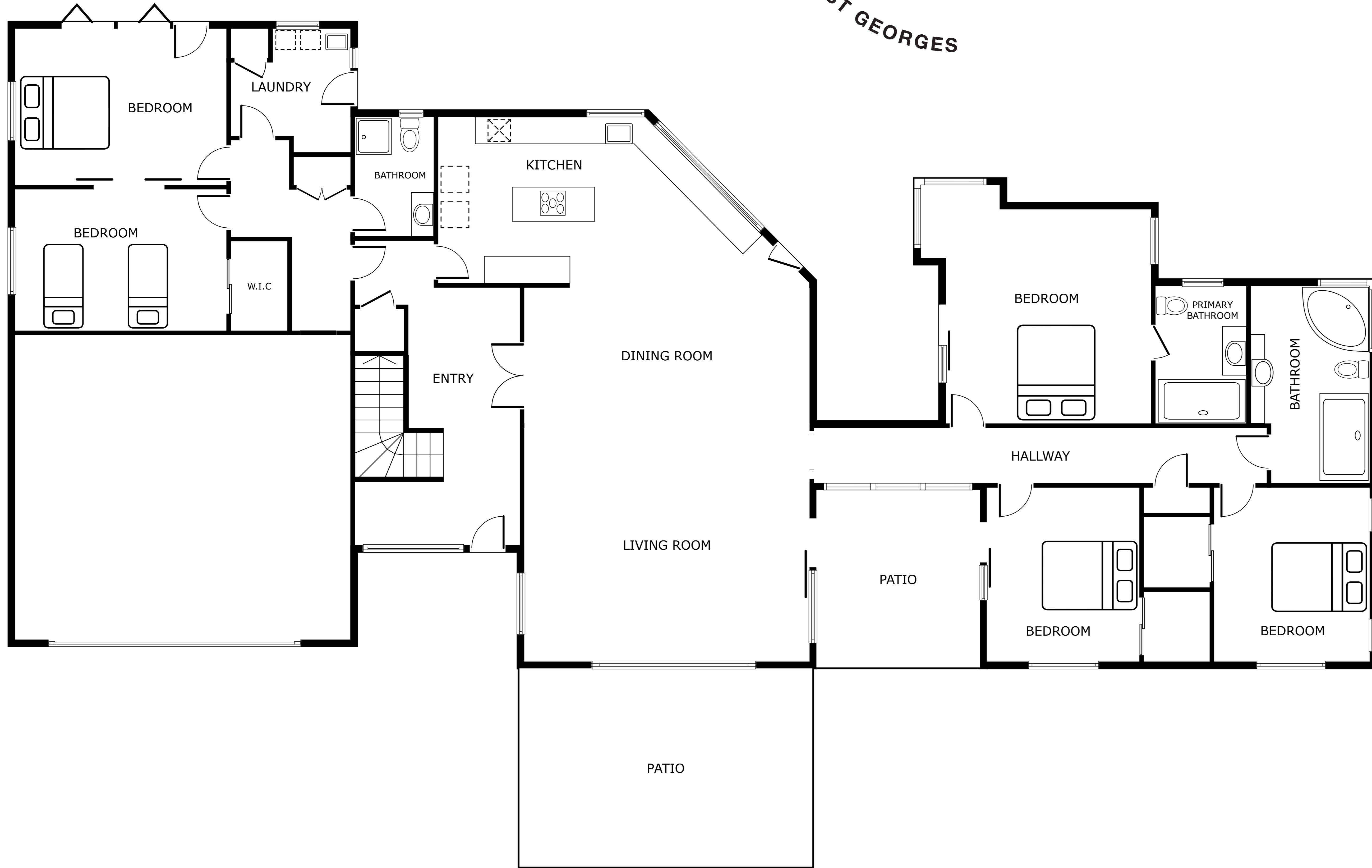
GROUND FLOOR
